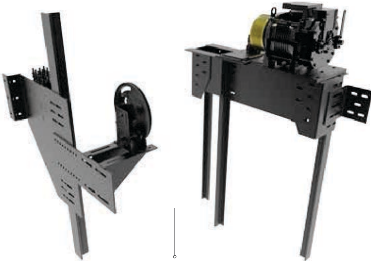
MRL MAKİNE ŞASESİ - MODEL 1 MRL MACHINE FRAME - MODEL 1
